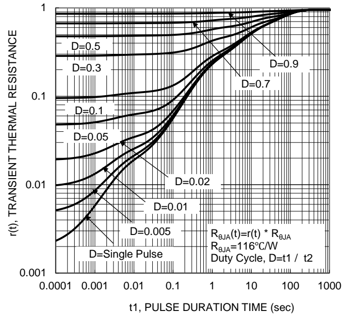
Figure 6. Transient Thermal Resistance
