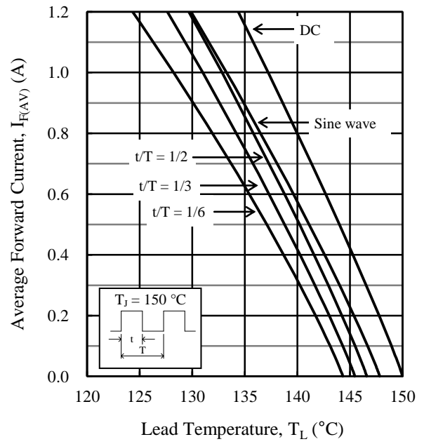
Figure 3. T_L vs. I_{F(AV)} Typical Characteristics ( V_R = 800\text{ V} )
